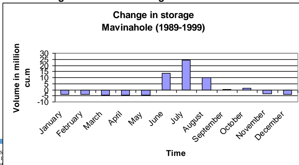
Figure 5.44: Water Budget - Mavinaholé
