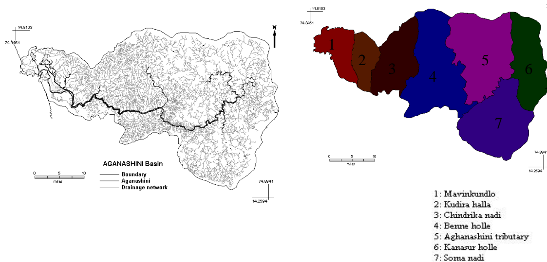
Fig. 2: Drainage network (a) and sub-basins (b) of the Aghanashini River basin
