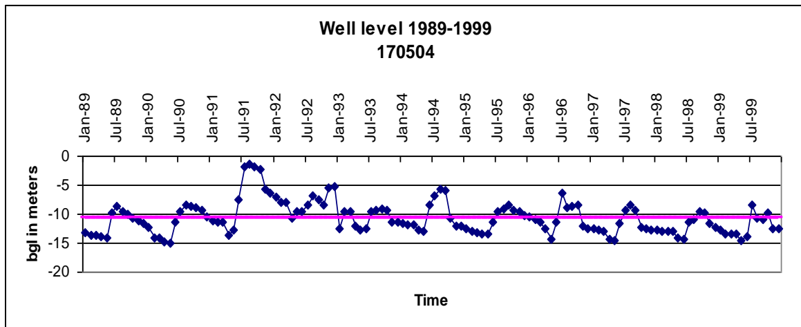
Figure 5.37 Water Table Depths (bgl) in Selected Wells Upstream (1989-1999)
